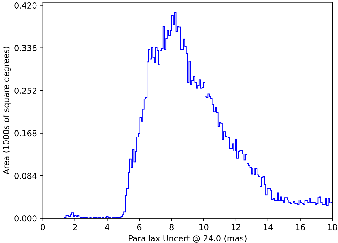
roll_pause_mjdp365_v3.4_10yrs All sky: Parallax Uncert @ 24.0
