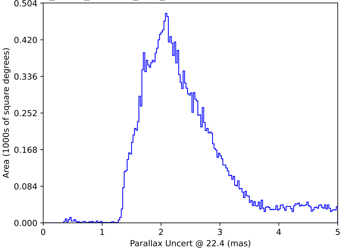
roll_pause_mjdp365_v3.4_10yrs All sky: Parallax Uncert @ 22.4
