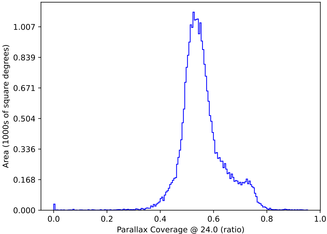
roll_pause_mjdp365_v3.4_10yrs All sky: Parallax Coverage @ 24.0
