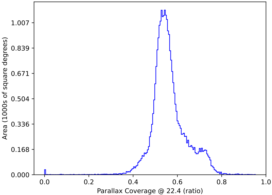
roll_pause_mjdp365_v3.4_10yrs All sky: Parallax Coverage @ 22.4
