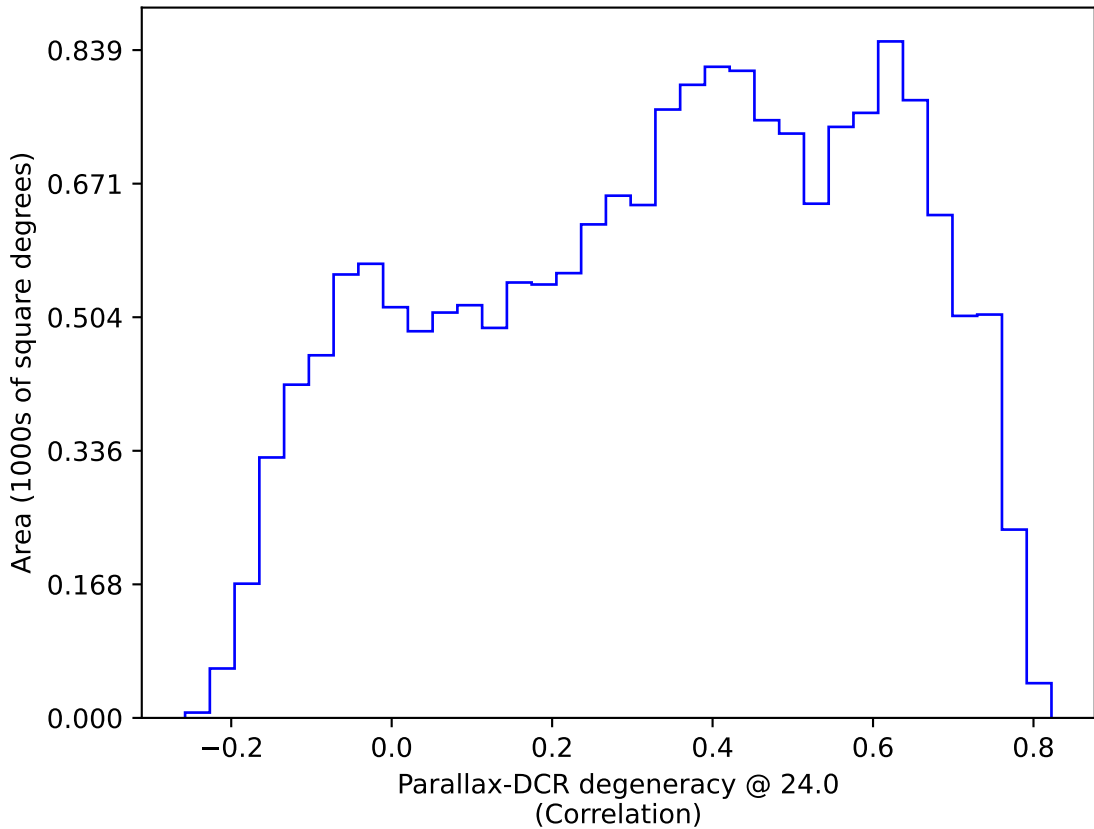
roll_pause_mjdp365_v3.4_10yrs WFD: Parallax-DCR degeneracy @ 24.0
