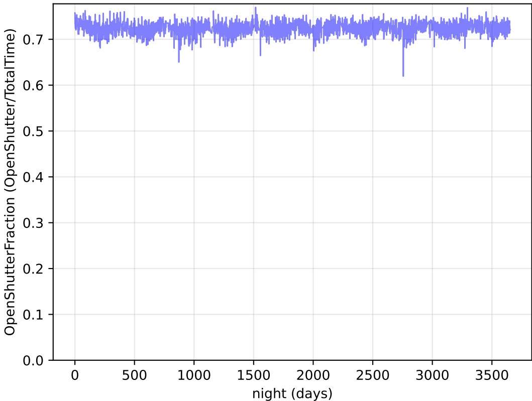
roll_pause_mjdp365_v3.4_10yrs Per night: OpenShutterFraction
