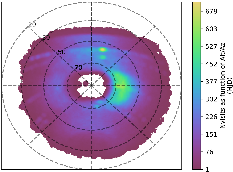
roll_pause_mjdp365_v3.4_10yrs u band: Nvisits as function of Alt/Az
