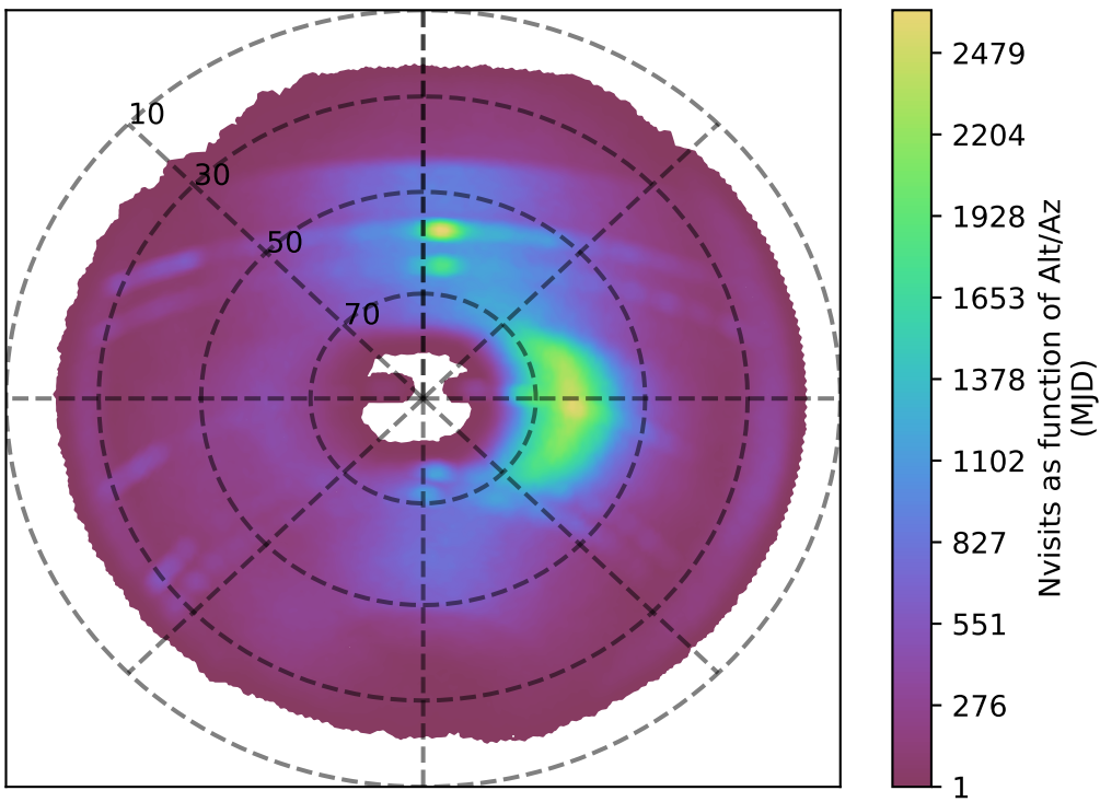
roll_pause_mjdp365_v3.4_10yrs i band: Nvisits as function of Alt/Az
