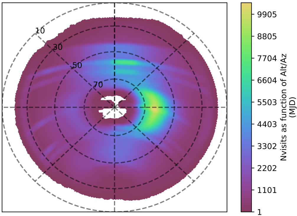
roll_pause_mjdp365_v3.4_10yrs all bands: Nvisits as function of Alt/Az
