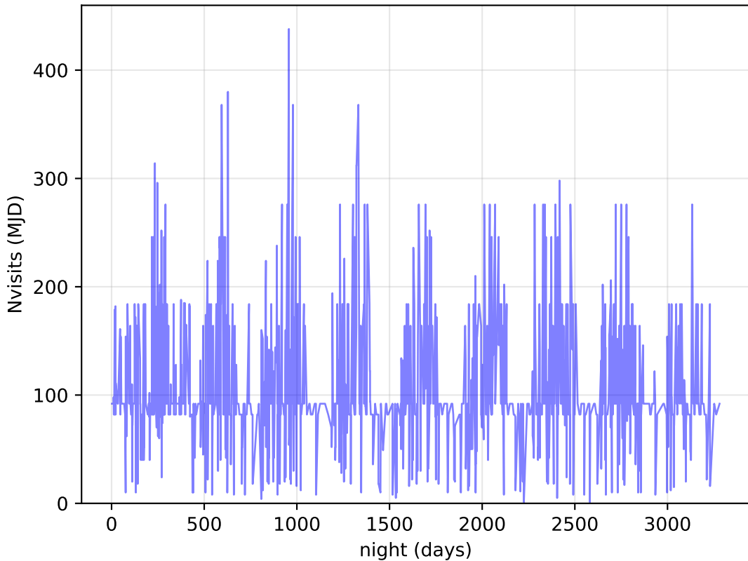
roll_pause_mjdp365_v3.4_10yrs DDF: Nvisits
