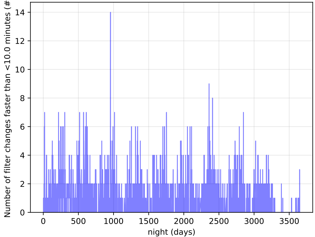
roll_pause_midp365_v3.4_10yrs Per Night: Number of filter changes faster than <10.0 minutes
