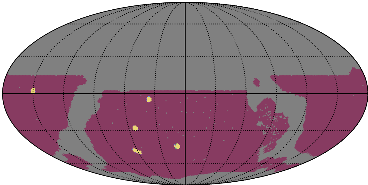
roll_pause_mjdp365_v3.4_10yrs WFD: NumberOfQuickRevisits
