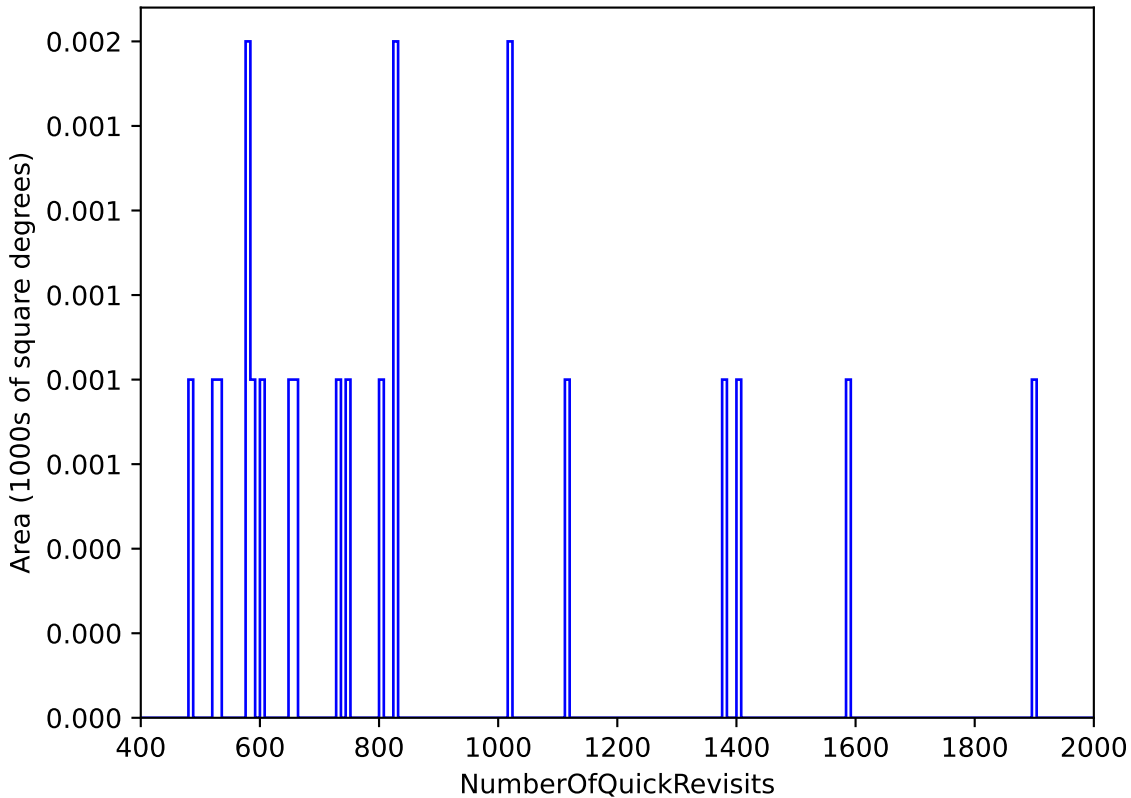
roll_pause_mjdp365_v3.4_10yrs WFD: NumberOfQuickRevisits
