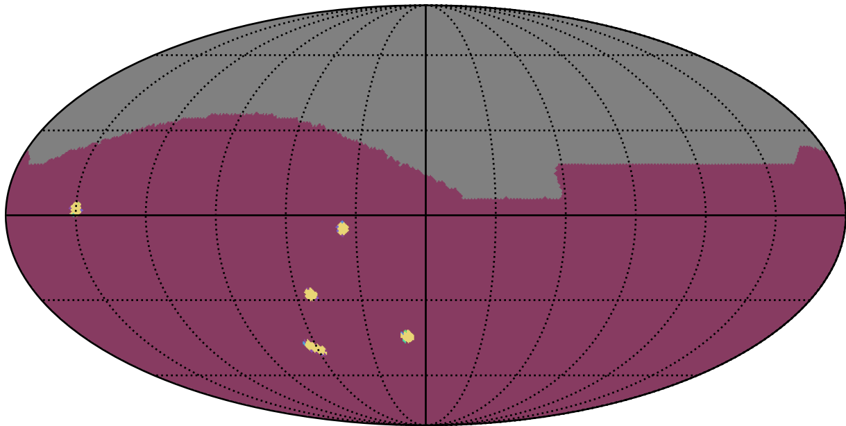
roll_pause_mjdp365_v3.4_10yrs All sky: NumberOfQuickRevisits
