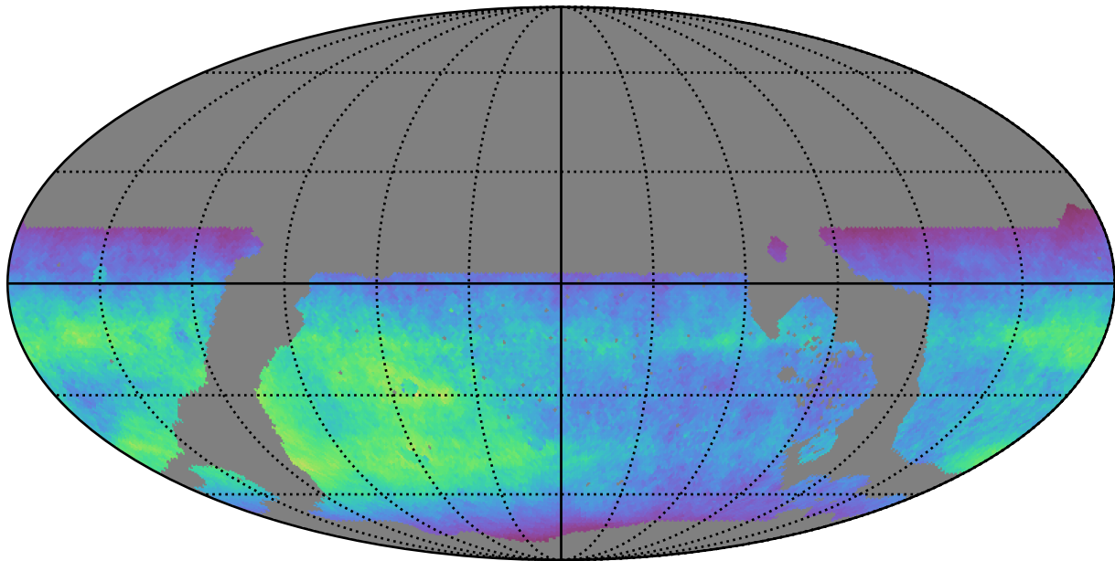
roll_pause_mjdp365_v3.4_10yrs WFD z band: Normalized Teff
