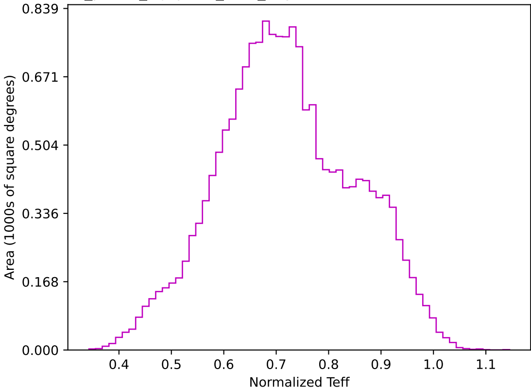
roll_pause_mjdp365_v3.4_10yrs WFD z band: Normalized Teff
