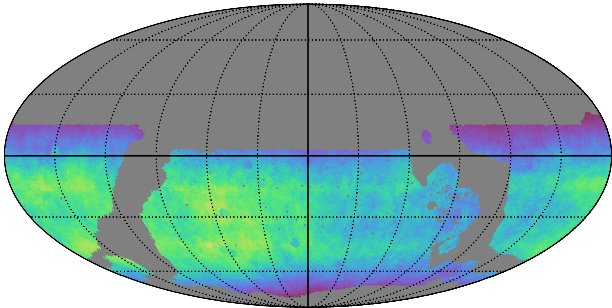
roll_pause_mjdp365_v3.4_10yrs WFD y band: Normalized Teff
