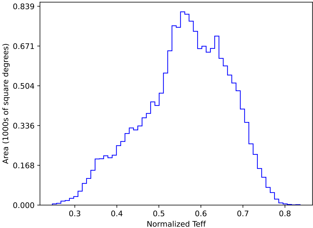
roll_pause_mjdp365_v3.4_10yrs WFD y band: Normalized Teff
