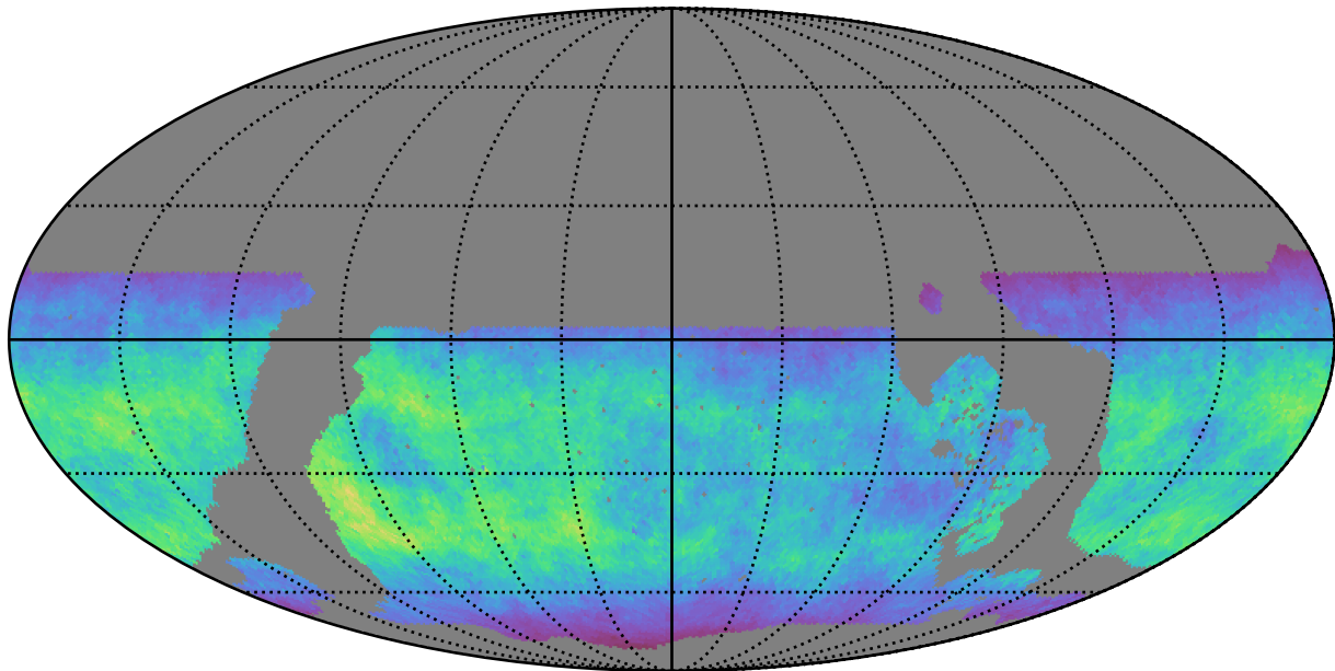
roll_pause_mjdp365_v3.4_10yrs WFD u band: Normalized Teff
