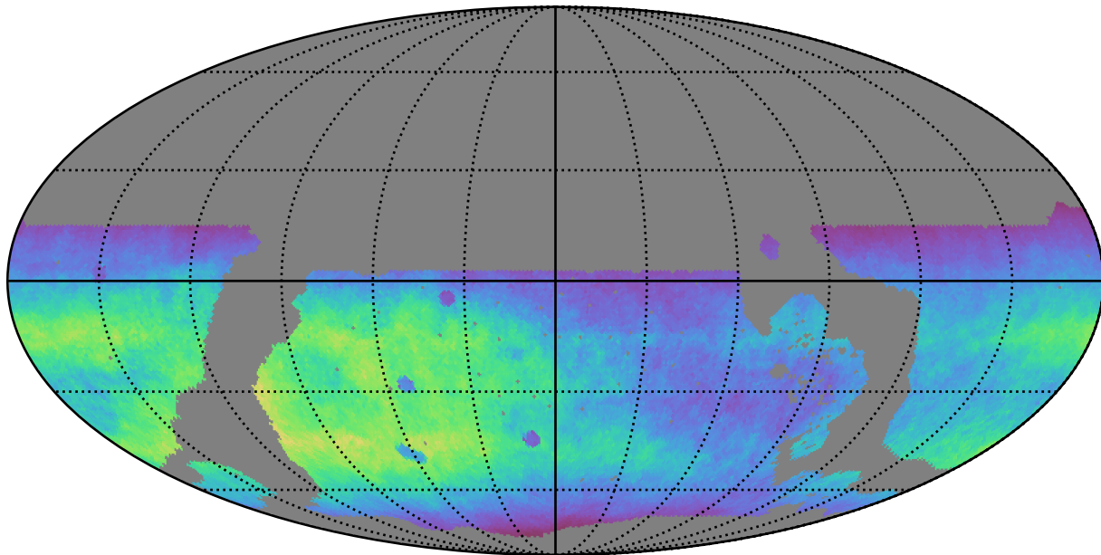
roll_pause_mjdp365_v3.4_10yrs WFD r band: Normalized Teff
