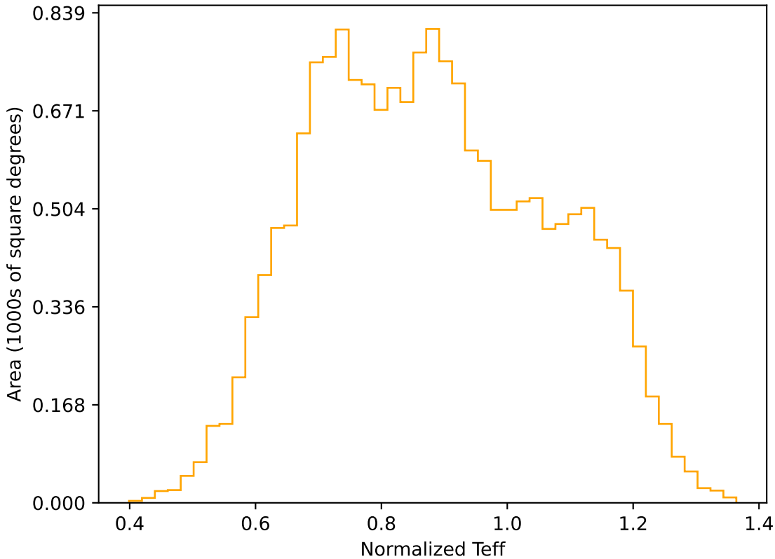
roll_pause_mjdp365_v3.4_10yrs WFD r band: Normalized Teff
