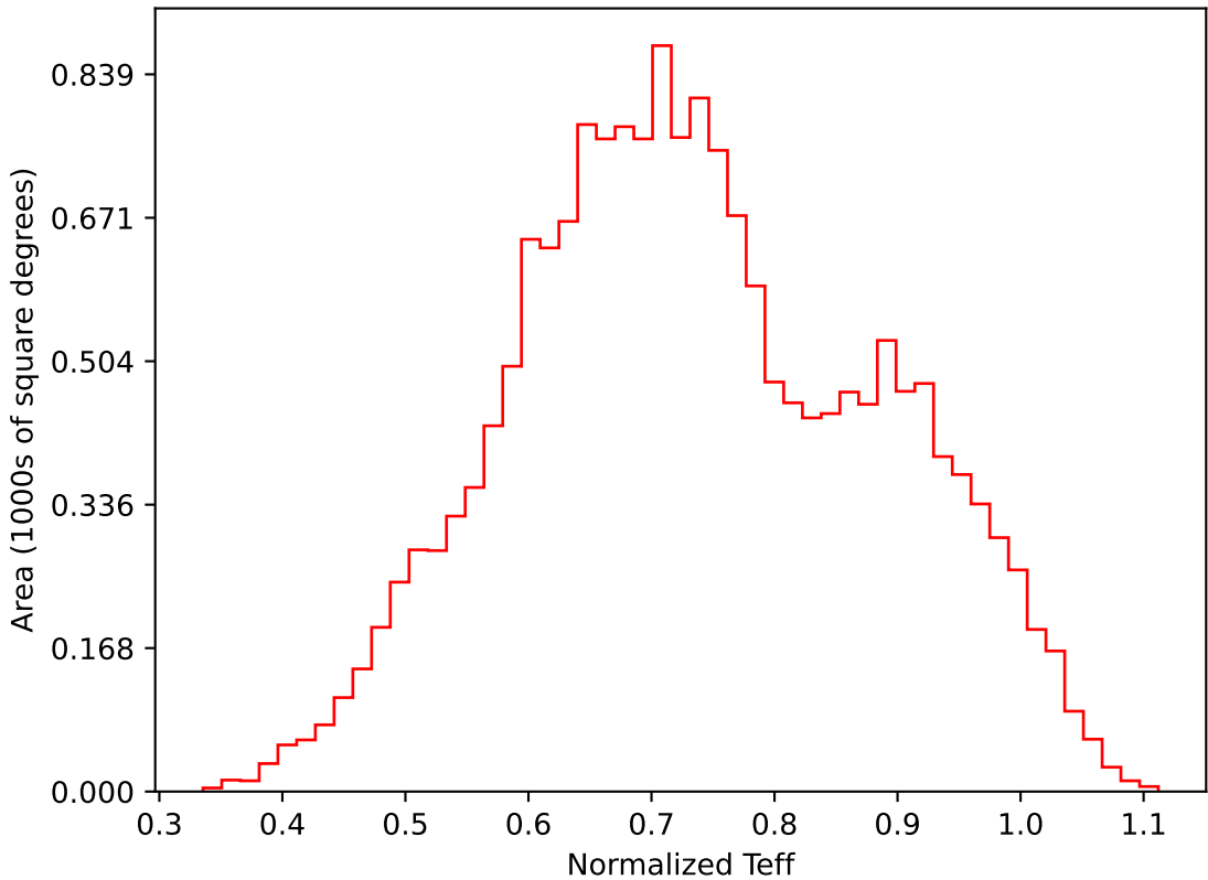
roll_pause_mjdp365_v3.4_10yrs WFD i band: Normalized Teff
