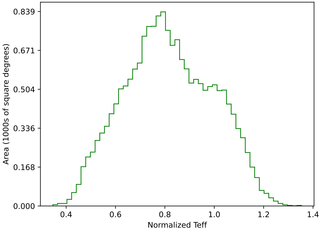
roll_pause_mjdp365_v3.4_10yrs WFD g band: Normalized Teff
