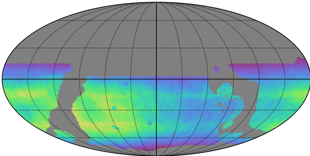
roll_pause_mjdp365_v3.4_10yrs WFD all bands: Normalized Teff
