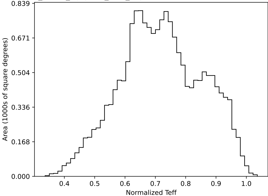
roll_pause_mjdp365_v3.4_10yrs WFD all bands: Normalized Teff
