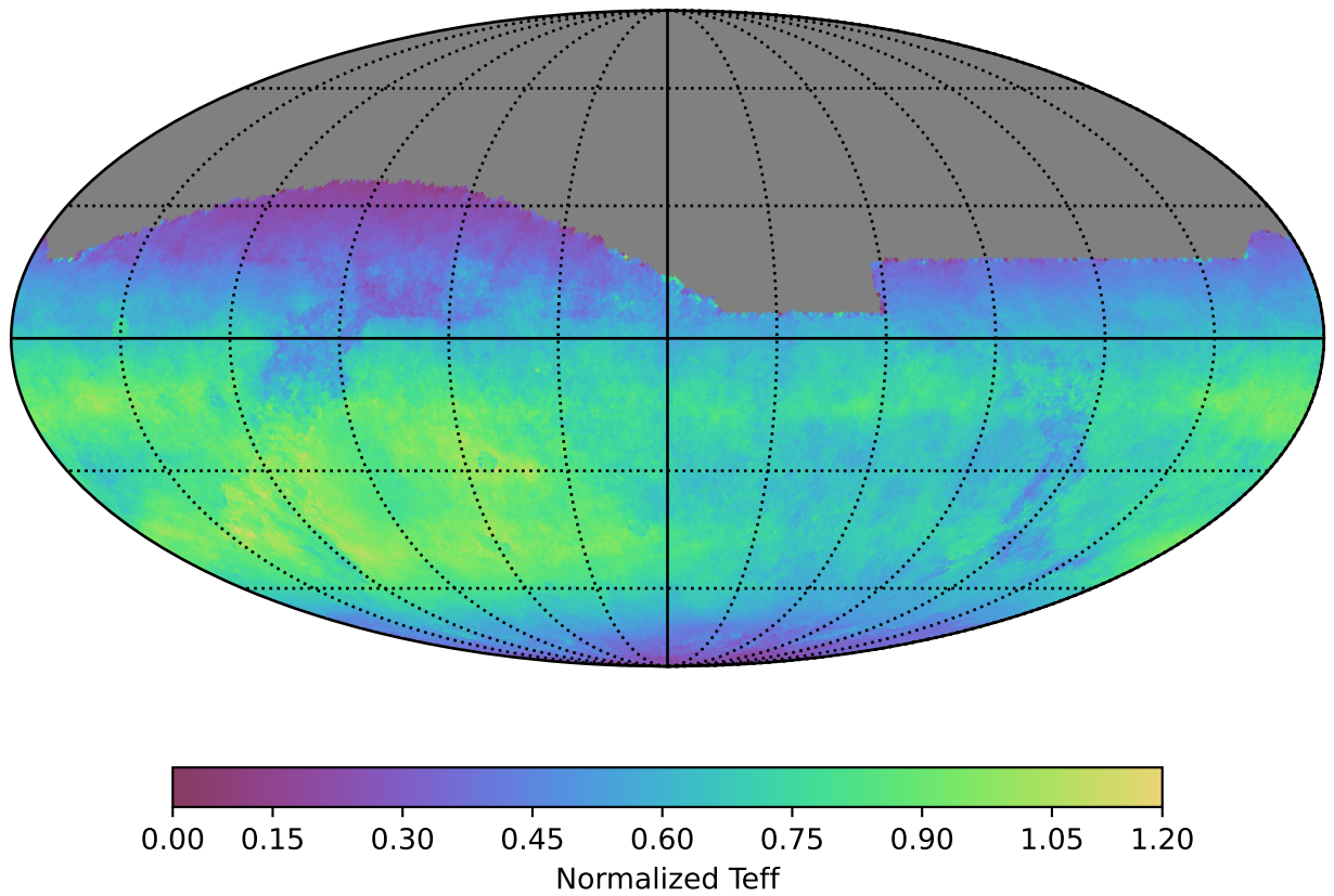
roll_pause_mjdp365_v3.4_10yrs All sky z band: Normalized Teff
