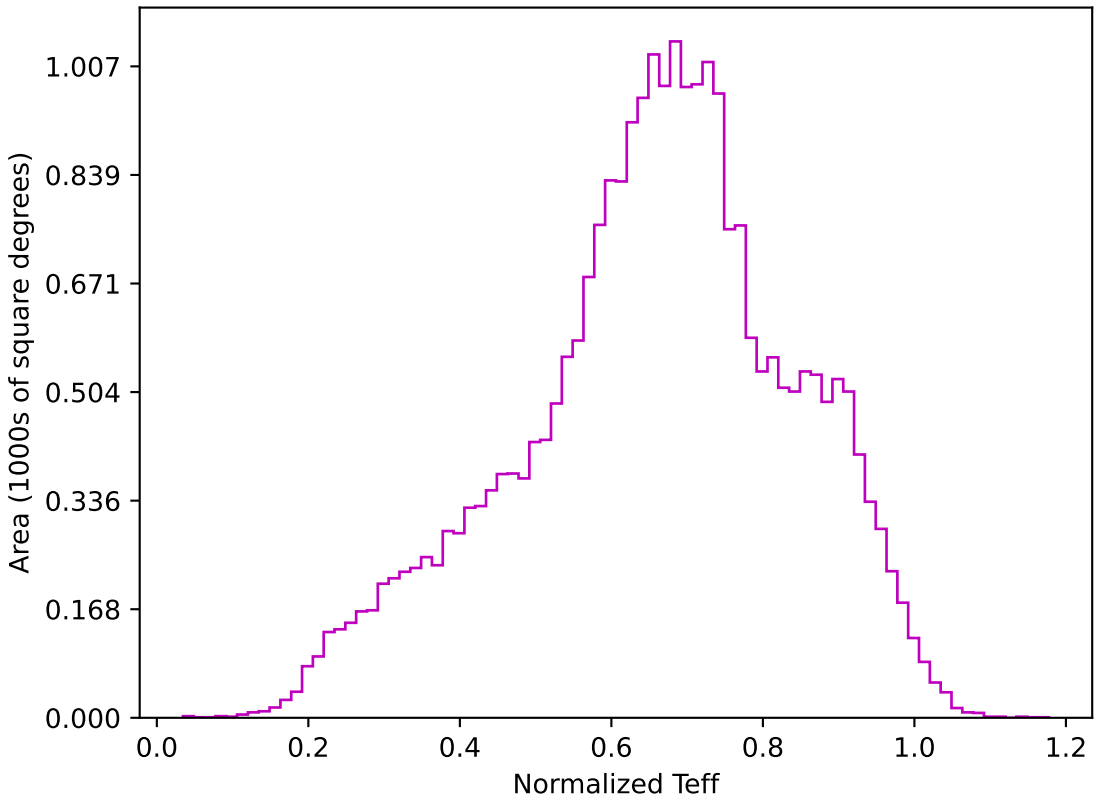
roll_pause_mjdp365_v3.4_10yrs All sky z band: Normalized Teff
