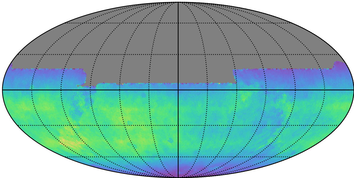
roll_pause_mjdp365_v3.4_10yrs All sky y band: Normalized Teff
