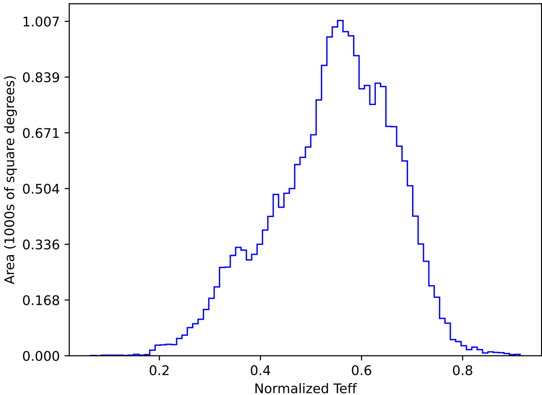
roll_pause_mjdp365_v3.4_10yrs All sky y band: Normalized Teff
