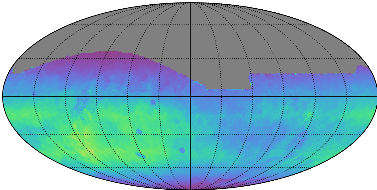
roll_pause_mjdp365_v3.4_10yrs All sky r band: Normalized Teff
