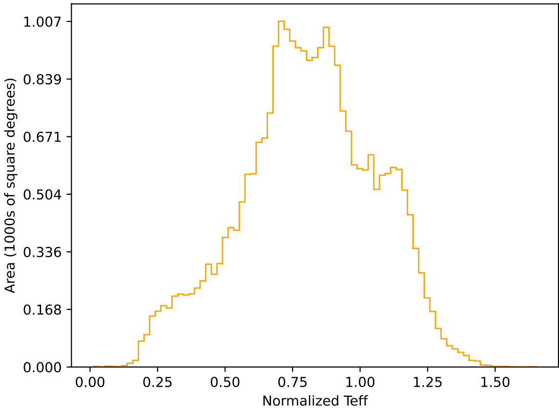
roll_pause_mjdp365_v3.4_10yrs All sky r band: Normalized Teff
