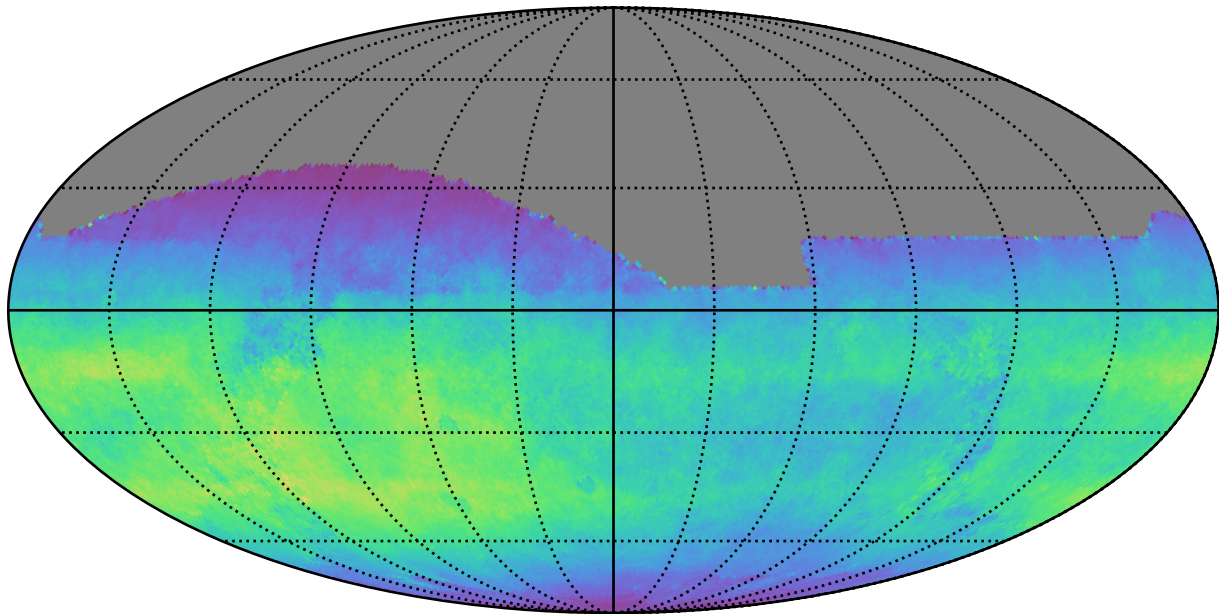
roll_pause_mjdp365_v3.4_10yrs All sky i band: Normalized Teff
