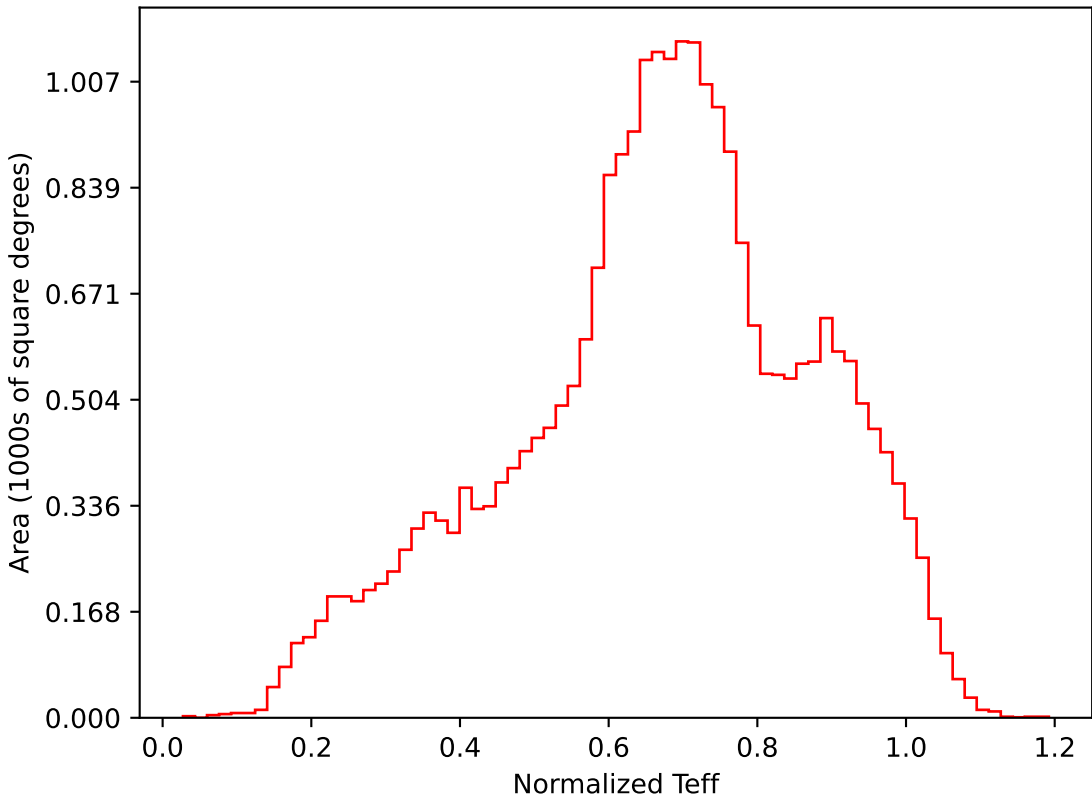
roll_pause_mjdp365_v3.4_10yrs All sky i band: Normalized Teff
