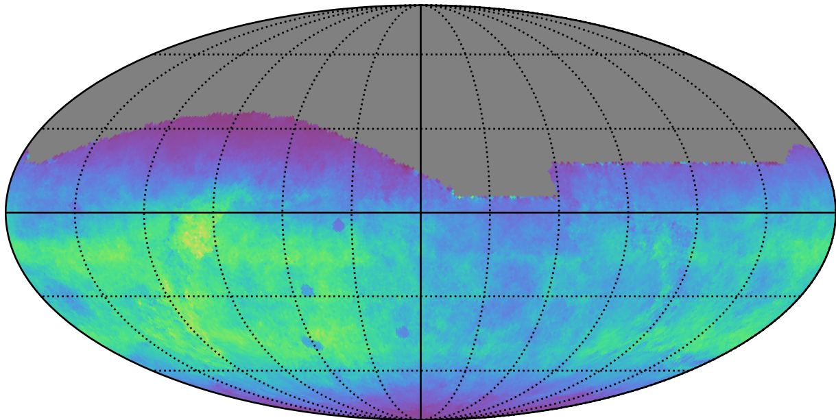
roll_pause_mjdp365_v3.4_10yrs All sky g band: Normalized Teff
