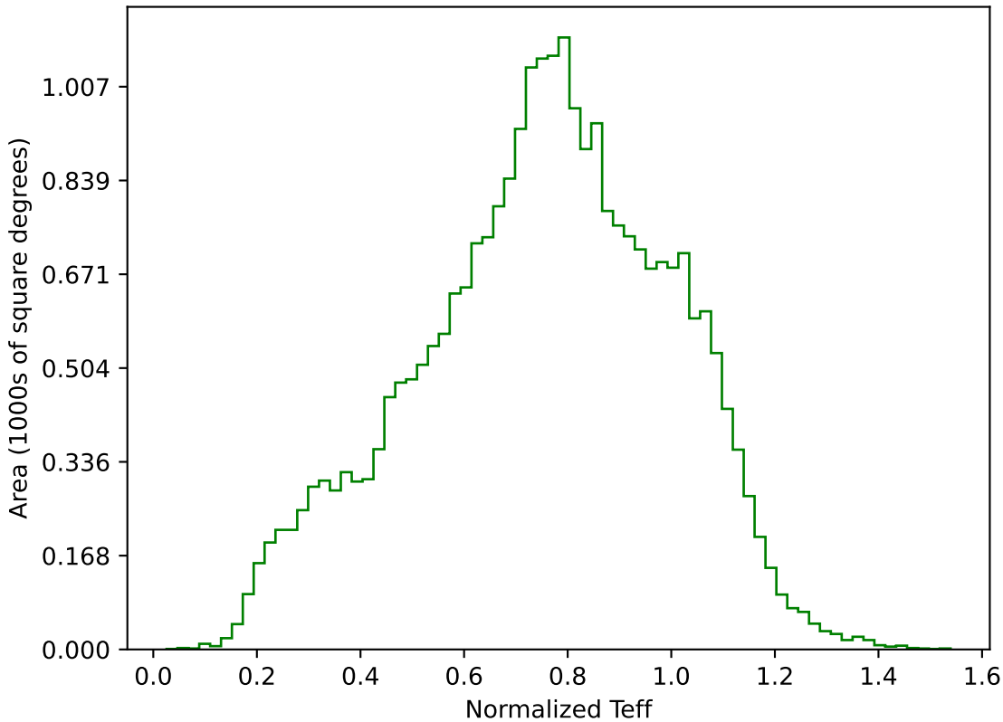
roll_pause_mjdp365_v3.4_10yrs All sky g band: Normalized Teff
