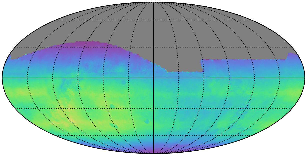
roll_pause_mjdp365_v3.4_10yrs All sky all bands: Normalized Teff
