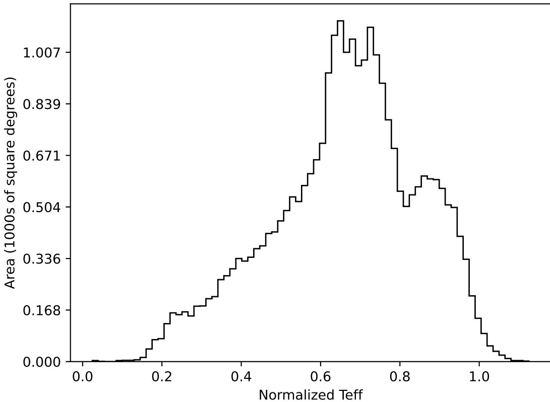
roll_pause_mjdp365_v3.4_10yrs All sky all bands: Normalized Teff
