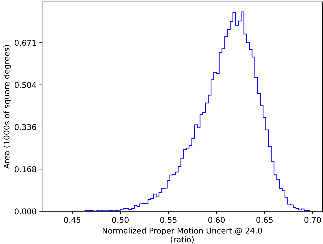
roll_pause_mjdp365_v3.4_10yrs WFD: Normalized Proper Motion Uncert @ 24.0
