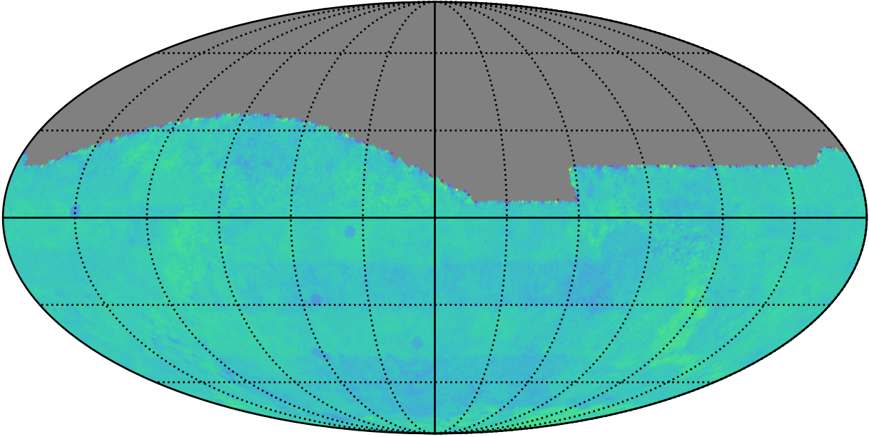
roll_pause_mjdp365_v3.4_10yrs All sky: Normalized Proper Motion Uncert @ 24.0
