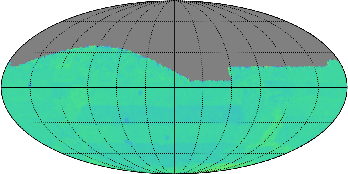
roll_pause_mjdp365_v3.4_10yrs All sky: Normalized Proper Motion Uncert @ 20.5
