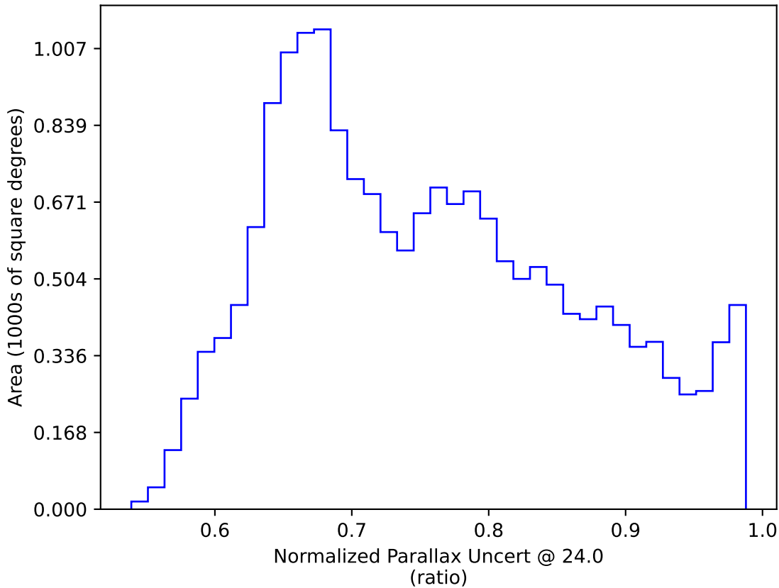
roll_pause_mjdp365_v3.4_10yrs WFD: Normalized Parallax Uncert @ 24.0
