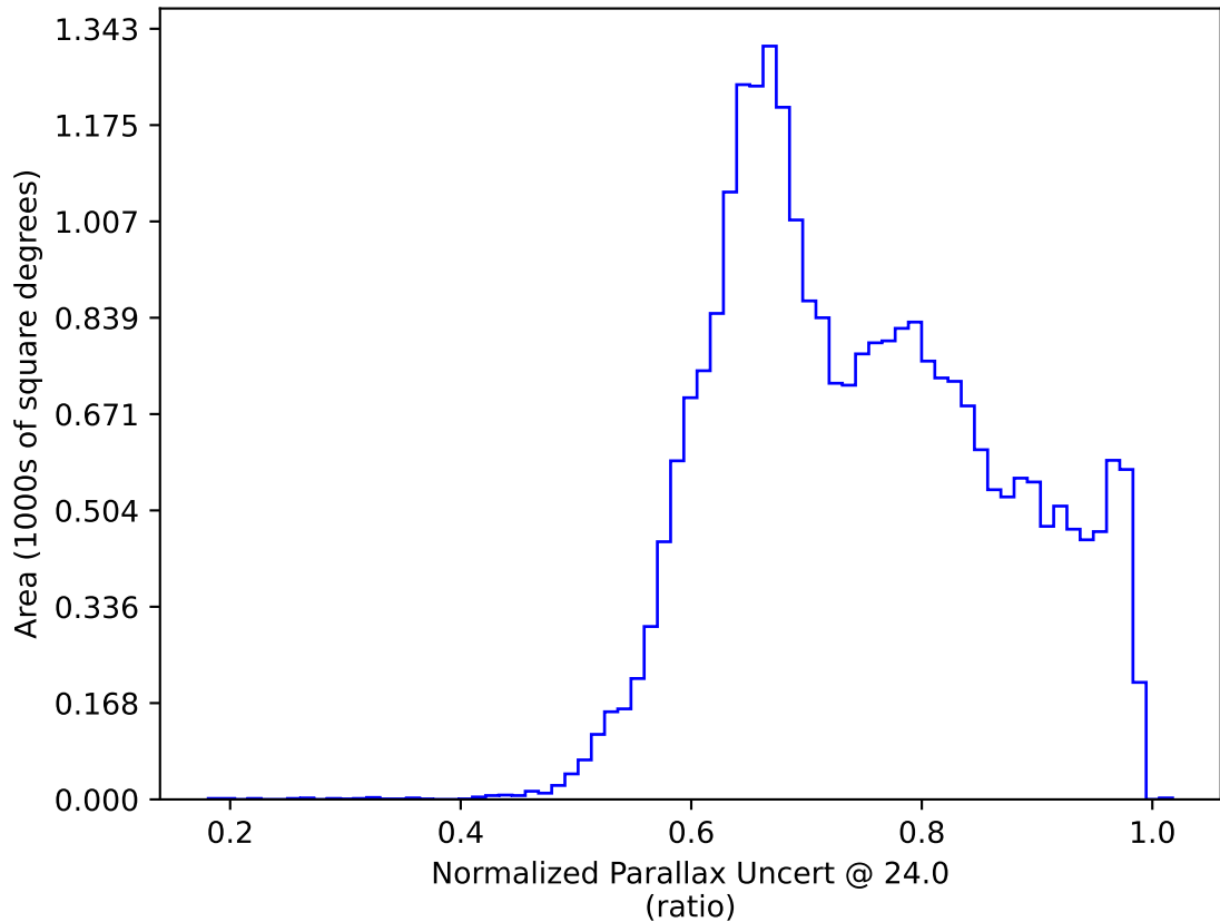
roll_pause_mjdp365_v3.4_10yrs All sky: Normalized Parallax Uncert @ 24.0
