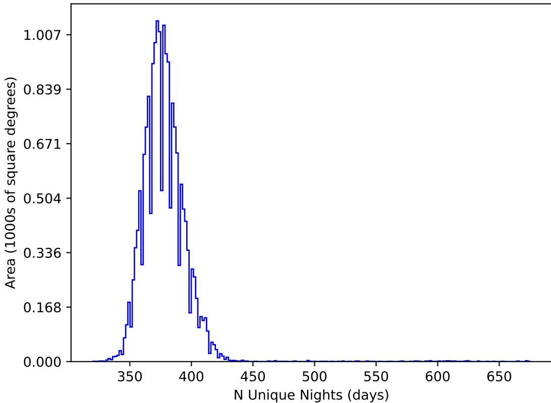
roll_pause_mjdp365_v3.4_10yrs WFD all bands: N Unique Nights
