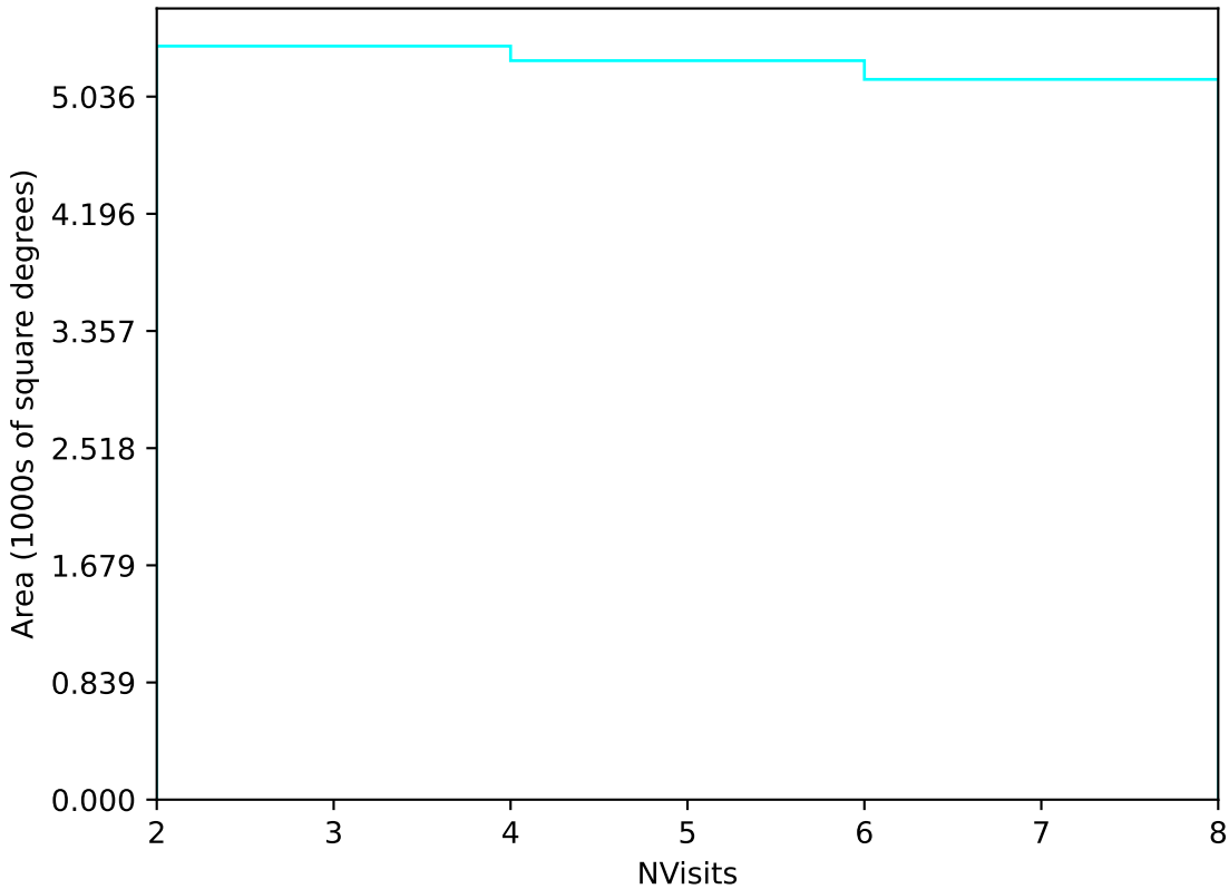
roll_pause_mjdp365_v3.4_10yrs Yr 3-4 u band: NVisits
