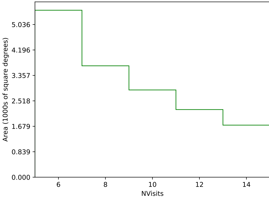
roll_pause_mjdp365_v3.4_10yrs Yr 3-4 g band: NVisits
