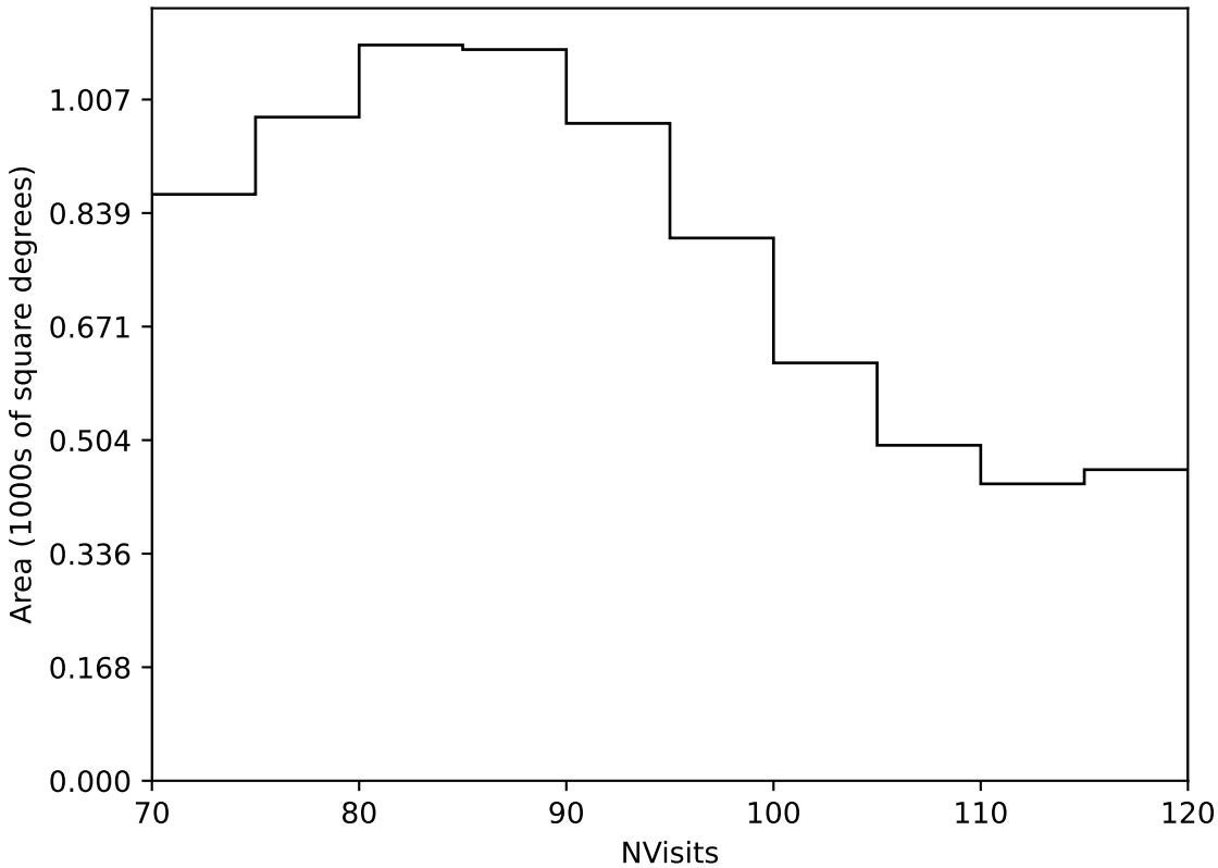
roll_pause_mjdp365_v3.4_10yrs Yr 3-4 all bands: NVisits
