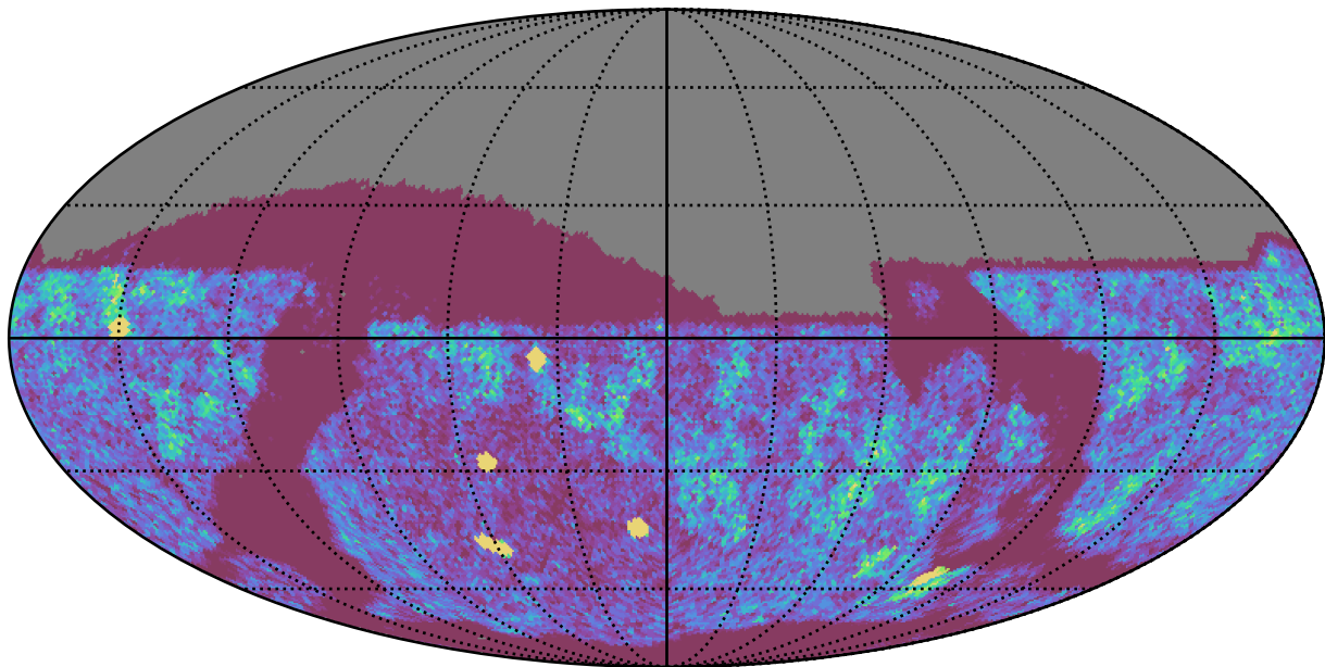
roll_pause_mjdp365_v3.4_10yrs Yr 1 z band: NVisits
