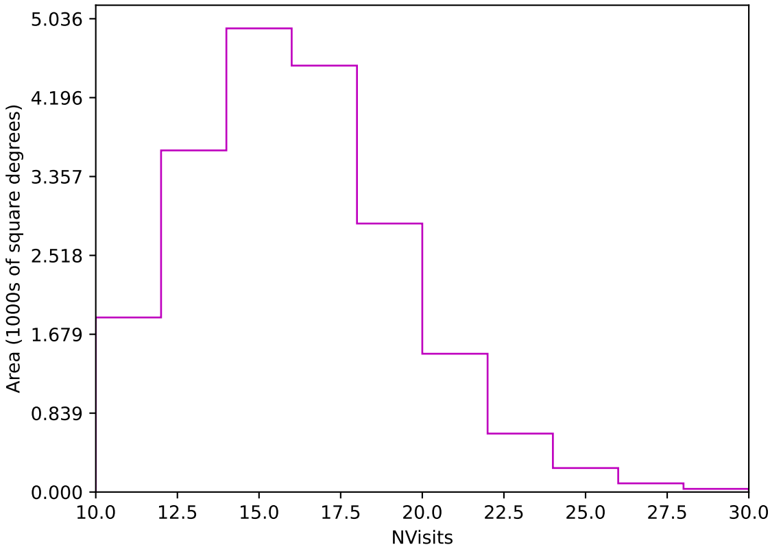
roll_pause_mjdp365_v3.4_10yrs Yr 1 z band: NVisits
