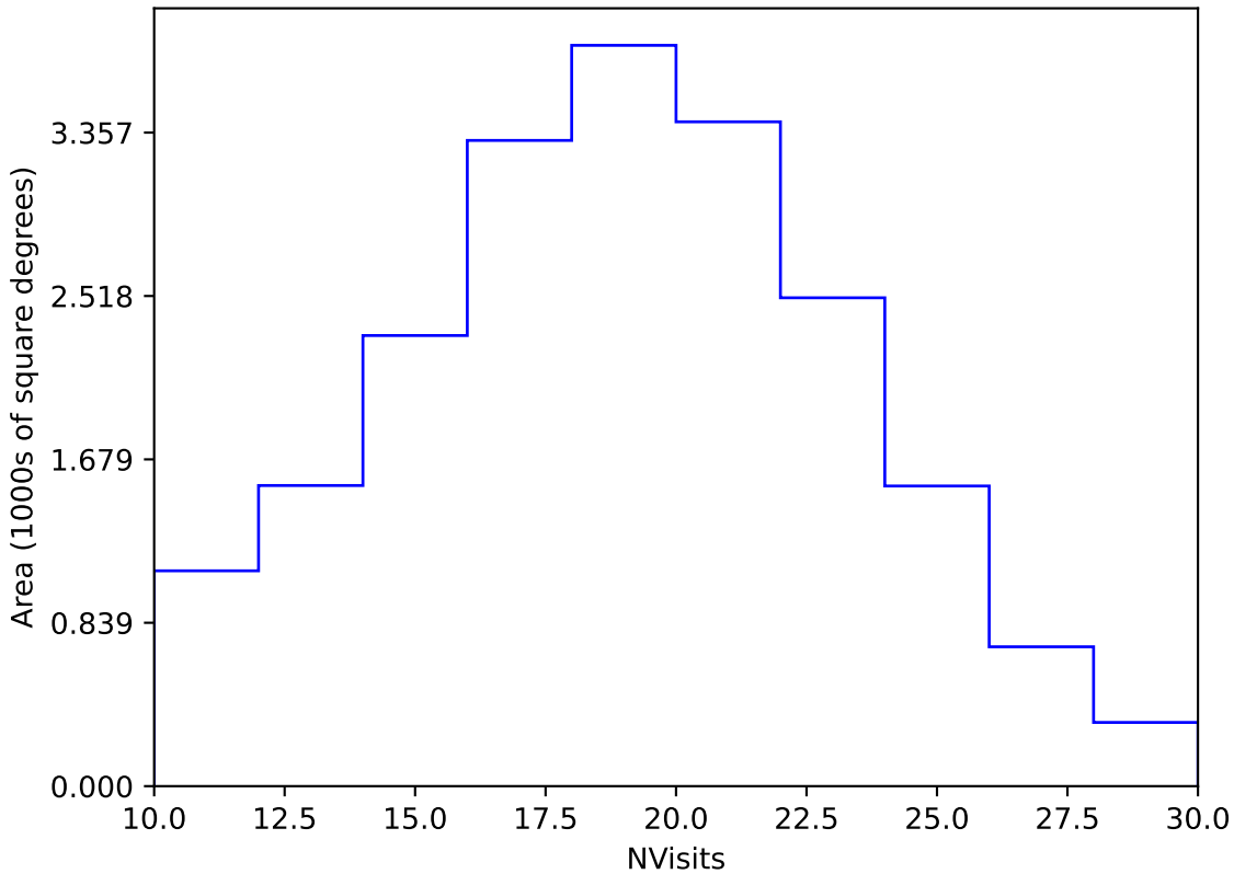
roll_pause_mjdp365_v3.4_10yrs Yr 1 y band: NVisits
