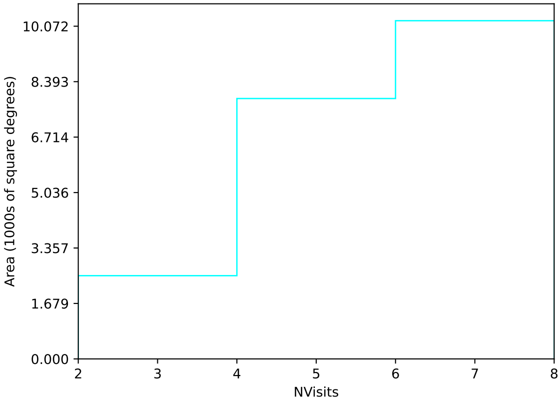
roll_pause_mjdp365_v3.4_10yrs Yr 1 u band: NVisits
